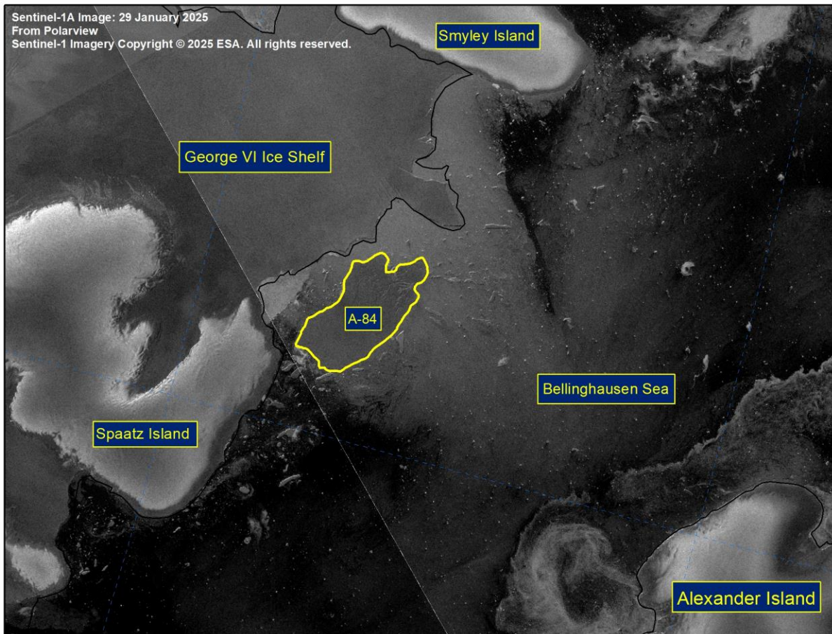
Figure 1: Sentinel-1 image of iceberg A-84 from January 29, 2025.
